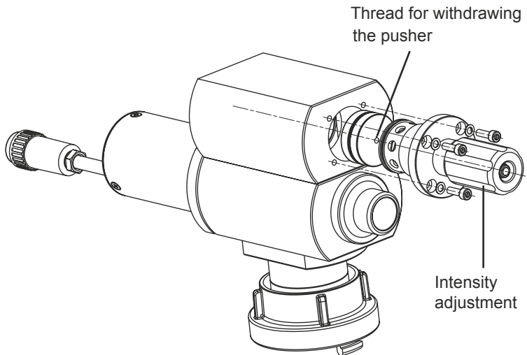
Picture 13: Stopper – cleaning the intensity adjustment
